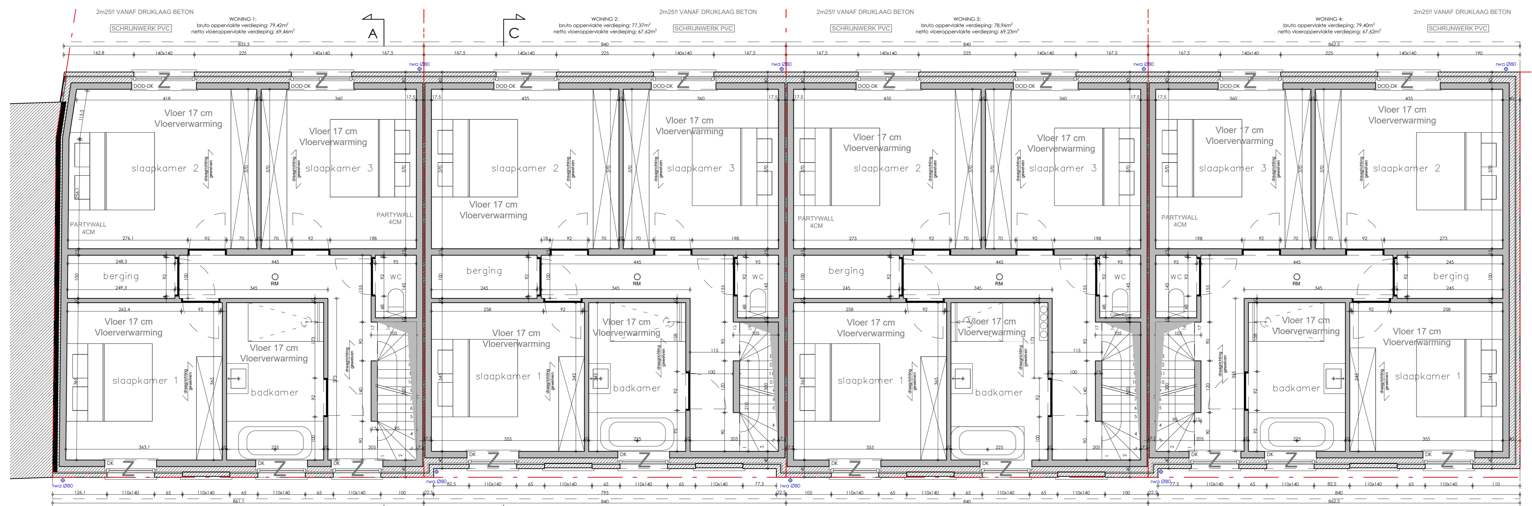
VERDIEPING +1 Schaal 1:50
